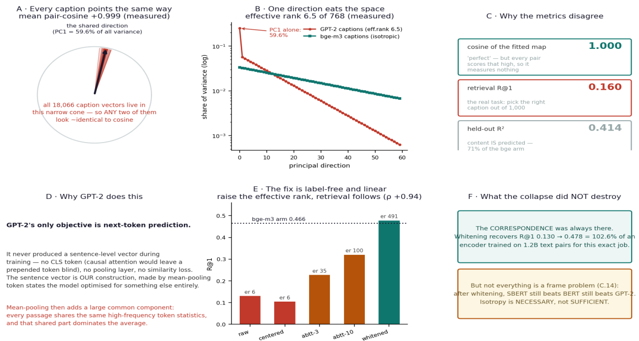
Figure C5b: the collapse and its spectrum, the metric disagreement it causes, its origin, the label-free fix, and what it does not destroy. The point cloud in panel A is schematic; every number shown is measured.
