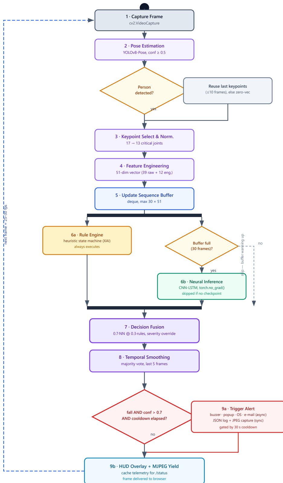
Figure 4.2 — Per-frame activity diagram. The rule engine (6a) always executes; the neural branch (6b) is skipped while the sequence buffer is still filling. Both branches join before fusion, and the whole activity repeats for the next captured frame.
