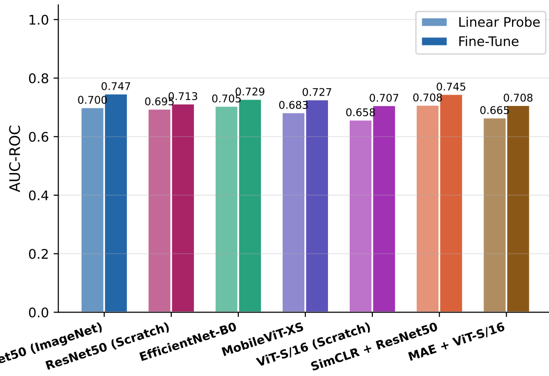
AUC-ROC: Linear Probe vs Fine-Tune (ChestX6 → ChestMNIST)
