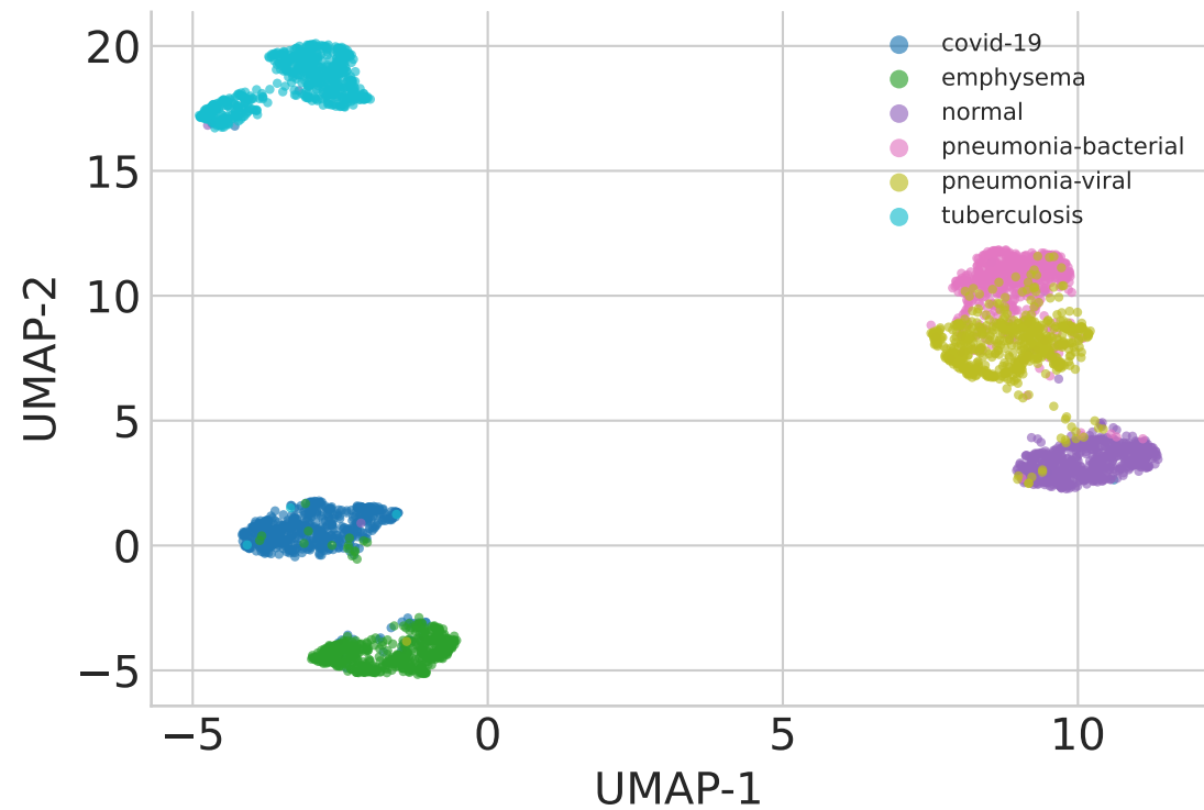
SimCLR + ResNet50 Silhouette: 0.642
