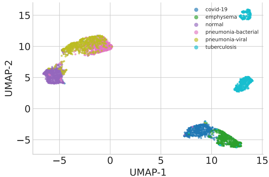
ResNet50 (Scratch) Silhouette: 0.420
