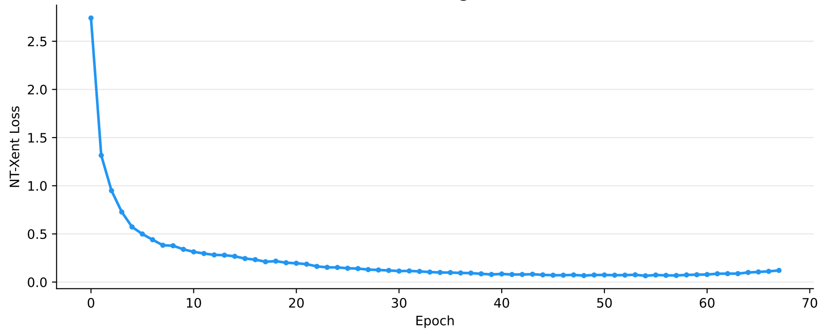
SimCLR Pretraining Loss Curve
