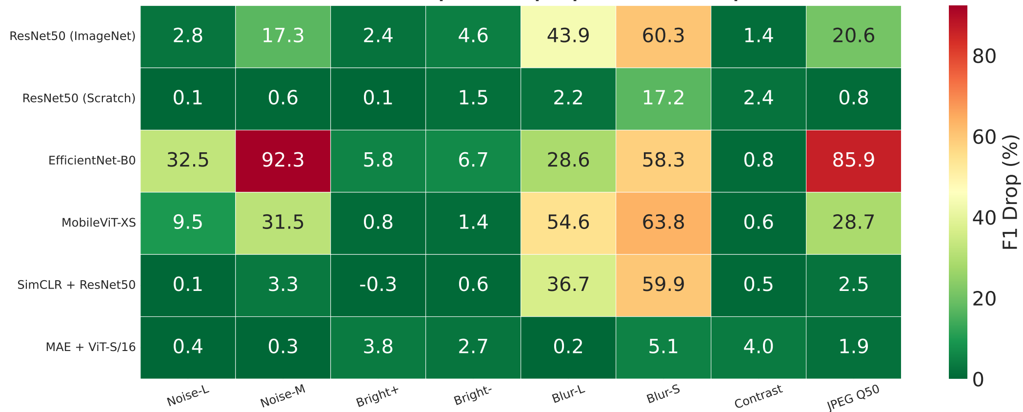
Robustness Heatmap — F1 Drop % per Model × Corruption
