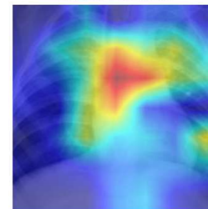
SimCLR + ResNet50
