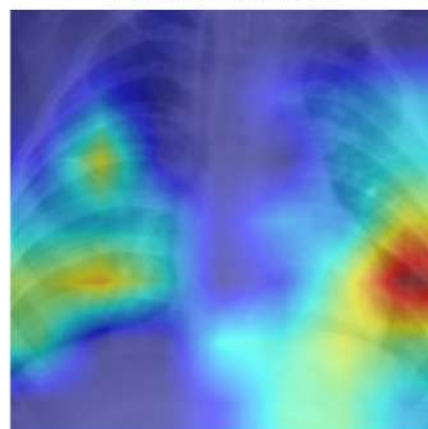
ResNet50 (Scratch)
