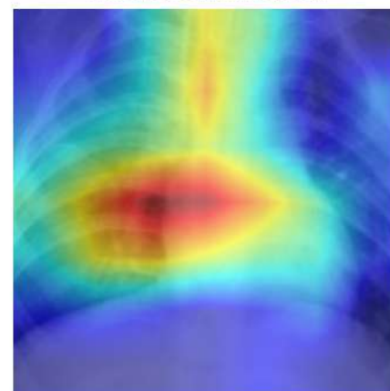
ResNet50 (ImageNet)
