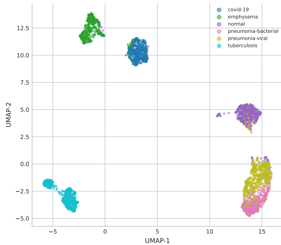
MobileViT-XS Silhouette: 0.607
