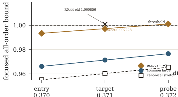
(c) Consecutive exact radius controls
