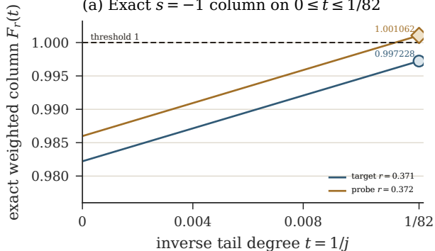
(a) Exact s = -1 column on 0 \leq t \leq 1/82
