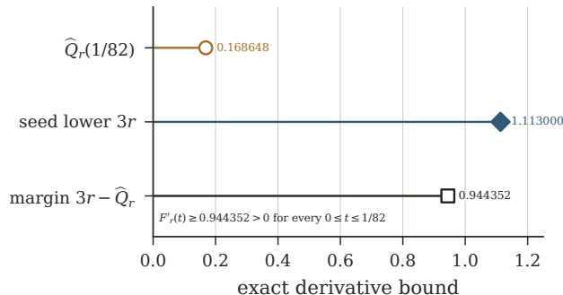
(b) Derivative lower bound at r = 0.371
