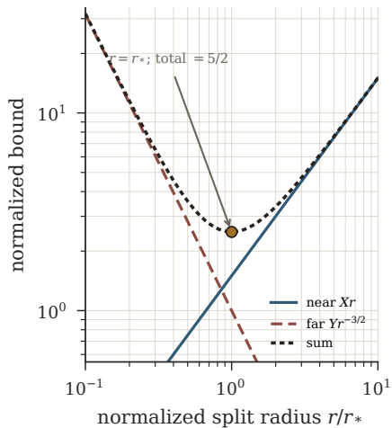
a Cancellation meets the far field
