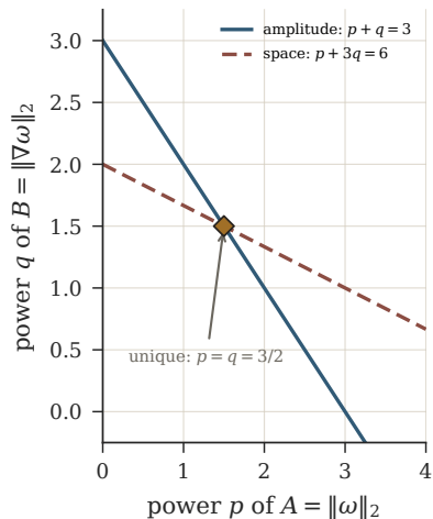
b Scaling fixes both exponents
