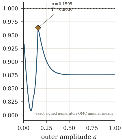
a Full-annulus screen
