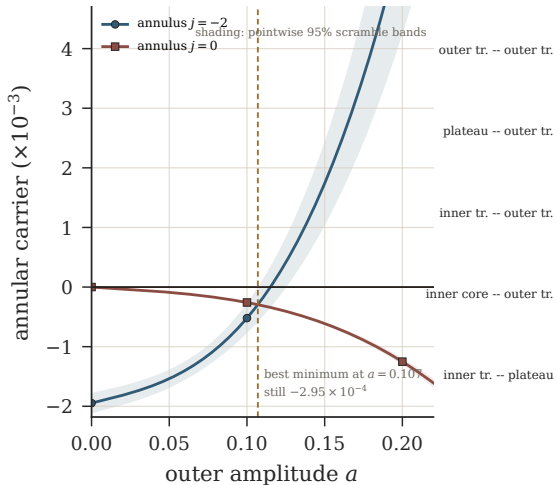
b Coarse-annulus root gap
