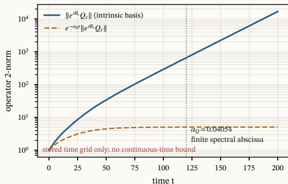
C Intrinsic moving-complement semigroup diagnostic
