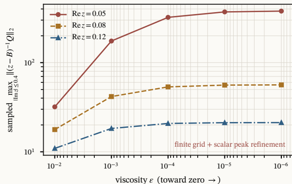
B Sampled vertical-line Q-resolvent peaks
