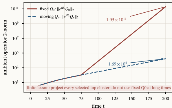
D A fixed inviscid complement leaks into the leading mode
