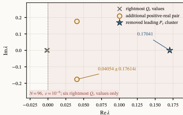
A Rightmost finite spectrum after one-cluster removal
