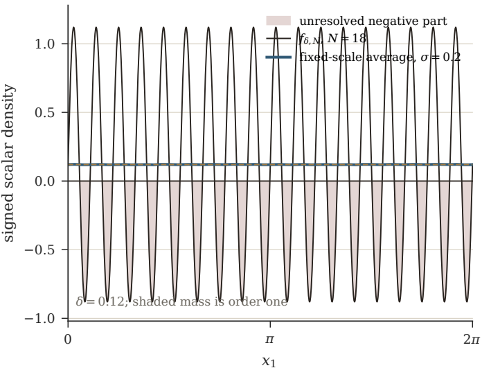
A Positive coarse view, negative fine mass
