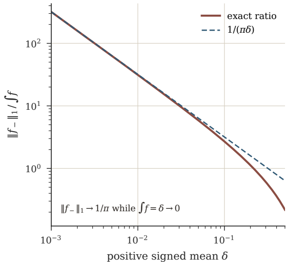
B Exact sign-defect separation
