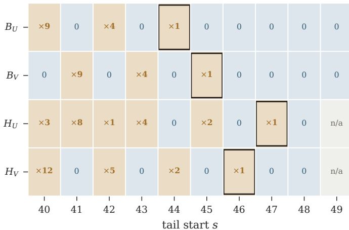
(b) Exact tail principal-minor scan
