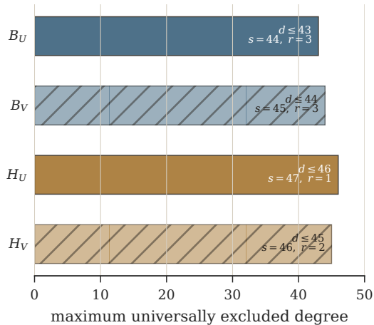
(a) Polynomial degree excluded
