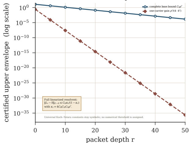
(b) Certified critical envelopes
