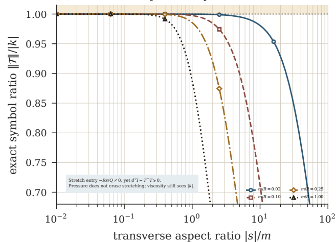
(a) Non-normal symbol stays below the derivative scale
