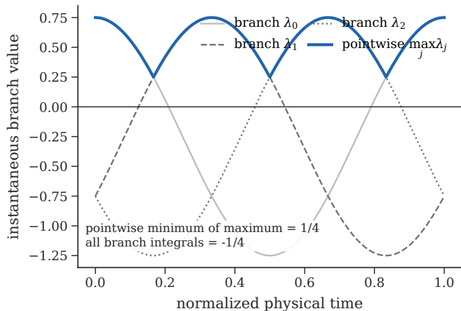
D Exact rotating-edge trap
