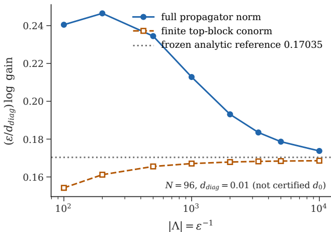
C Exact nonnormal prefactor trap
