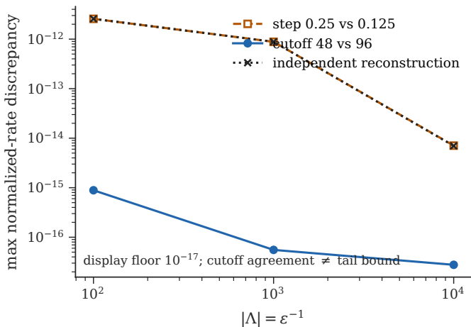
D Exact rotating-edge trap
