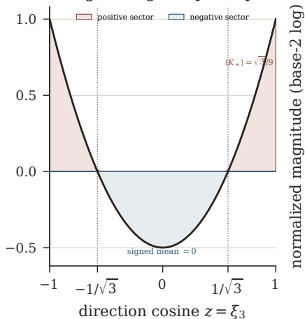
B Signed angular quadrupole
