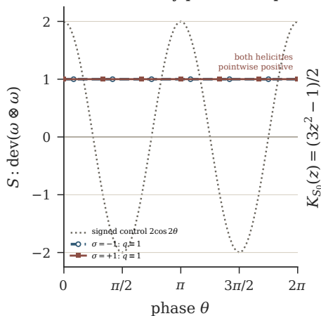
A Pure-helicity phase sweep
