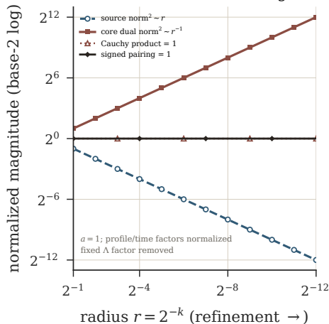
C Critical source-core ledger
