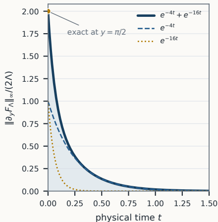
A Exact strain envelope
