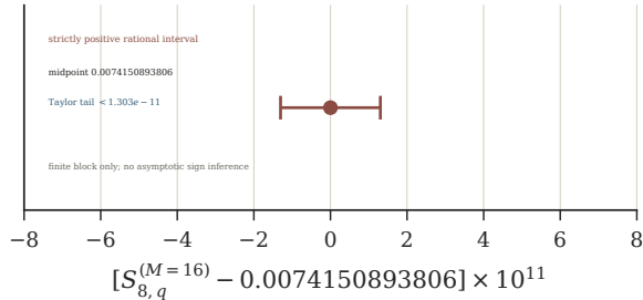
(b) Exact first-cycle heat enclosure
