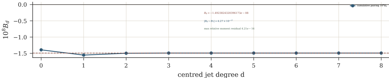
(c) The complete dominant heat-jet pairing stabilizes by degree eight
