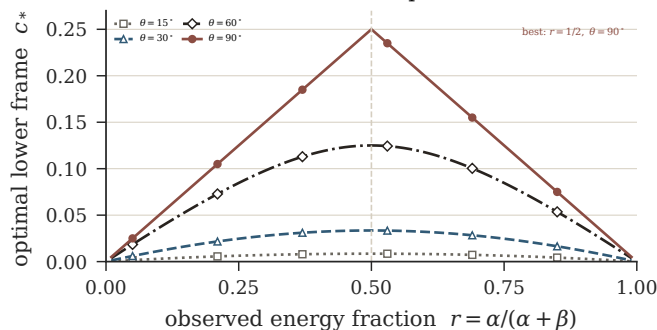
D More observations do not add directions
