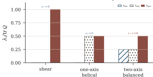
C Full rank, no uniform constant
