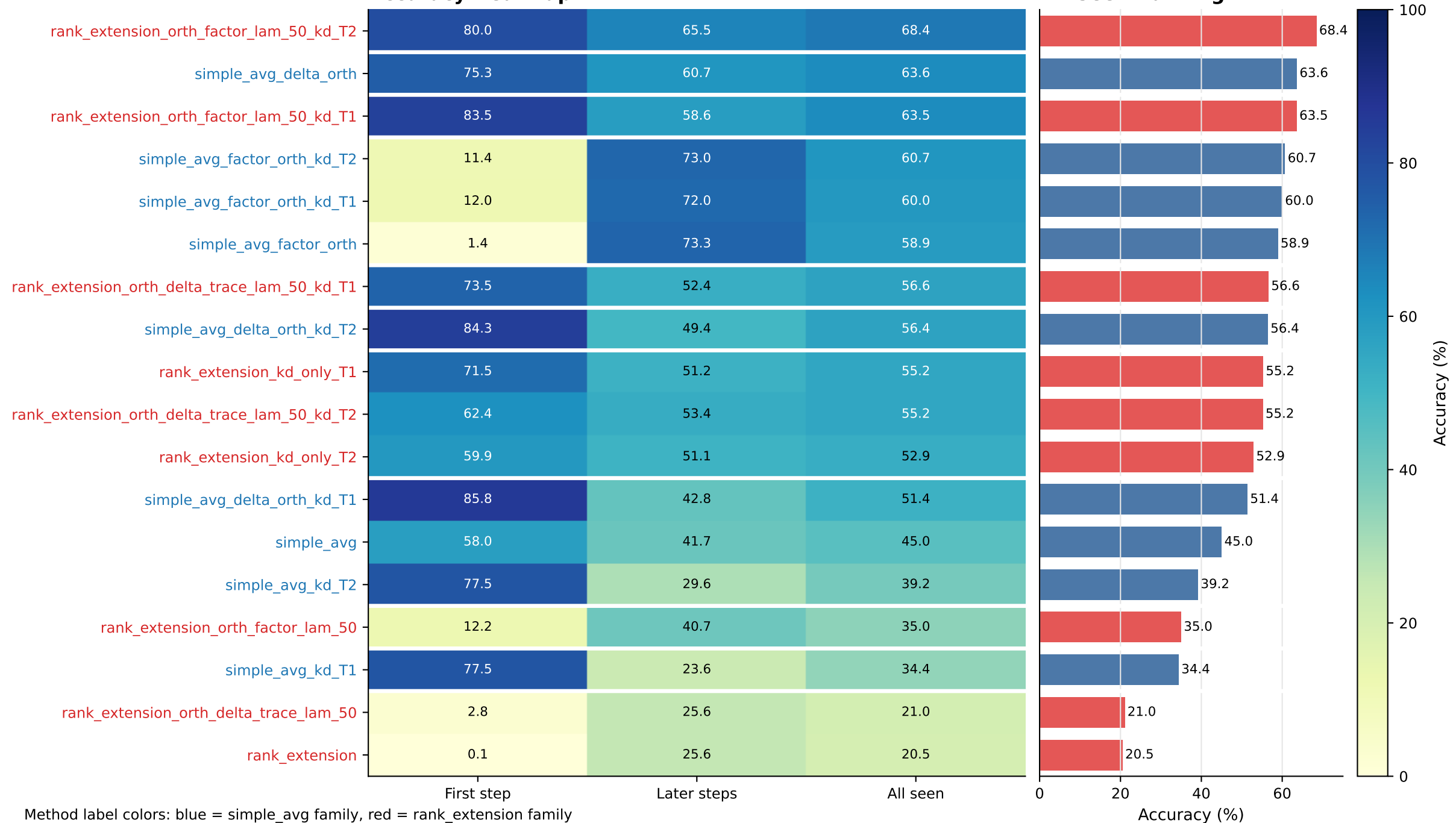
Accuracy Heatmap
