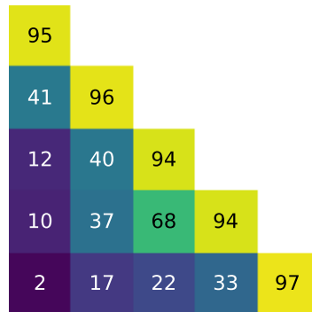
RankExt + FactorOrth
