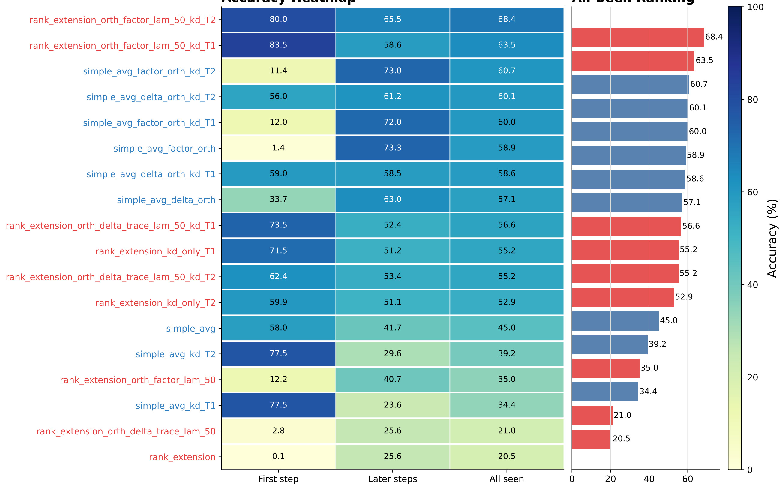
Accuracy Heatmap
