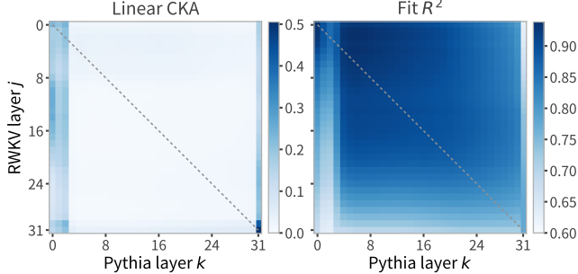
Fig. 2. All 32 \times 32 layer correspondences of raw residuals (generated from the canonical table paper_layer_correspondence.csv). Left: linear CKA is weak throughout, and high values concentrate in the row and column of layer 0 and the corner of the final layer — the diagonal (dashed) is not special. Right: the fit R^2 of per-layer linear maps fitted to the same pairs is high for nearly all pairs, at 0.62–0.94. The color scales of the two panels differ.
