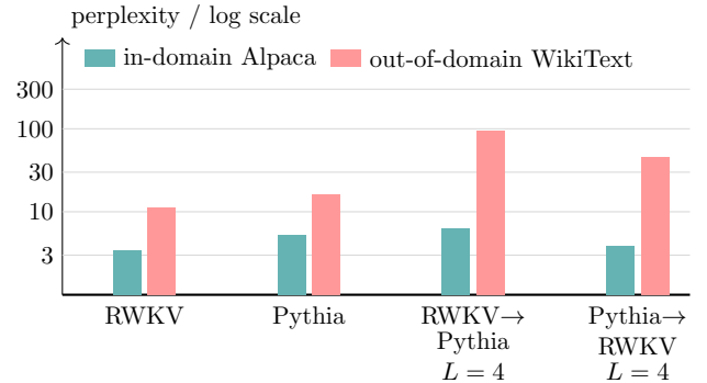
Fig. 6 Perplexity on Alpaca and WikiText-103 at context length 512. The vertical axis is logarithmic.
