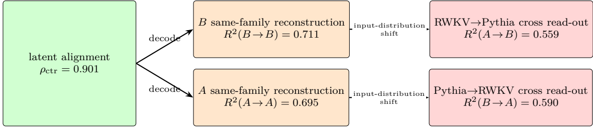
Fig. 3. The transition from the shared latent to the read-outs in both directions. High centered correlation coexists with imperfect self-reconstruction, and the RWKV \rightarrow Pythia/Pythia \rightarrow RWKV cross read-outs fall below, in all layers, the Pythia self-recon/RWKV self-recon self-reconstructions that use the same respective decoders.
