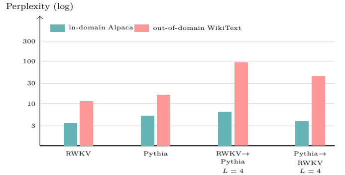
Fig. 6. Domain shift (context 512, log axis). Pythia→RWKV improves the WikiText perplexity of RWKV→Pythia ( L=4 ) from 93.87 \rightarrow 45.00 but does not reach the parents’ 11.33/16.22. Because the same adapter sits near the parents on Alpaca, domain, not length, is the primary difference.
