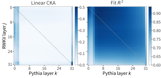
Fig. 2. All 32 \times 32 layer correspondences of raw residuals. Left: linear CKA is weak throughout, and high values concentrate in the row and column of layer 0 and the corner of the final layer — the diagonal (dashed) is not special. Right: the fit R^2 of per-layer linear maps fitted to the same pairs is high for nearly all pairs, at 0.62–0.94. The color scales of the two panels differ.
