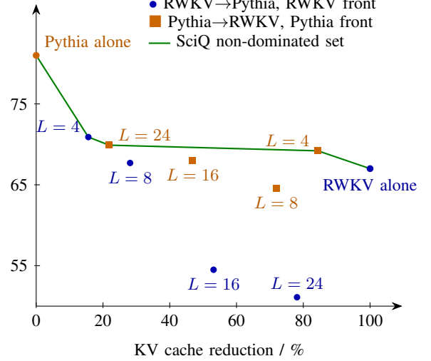
SciQ accuracy / %
