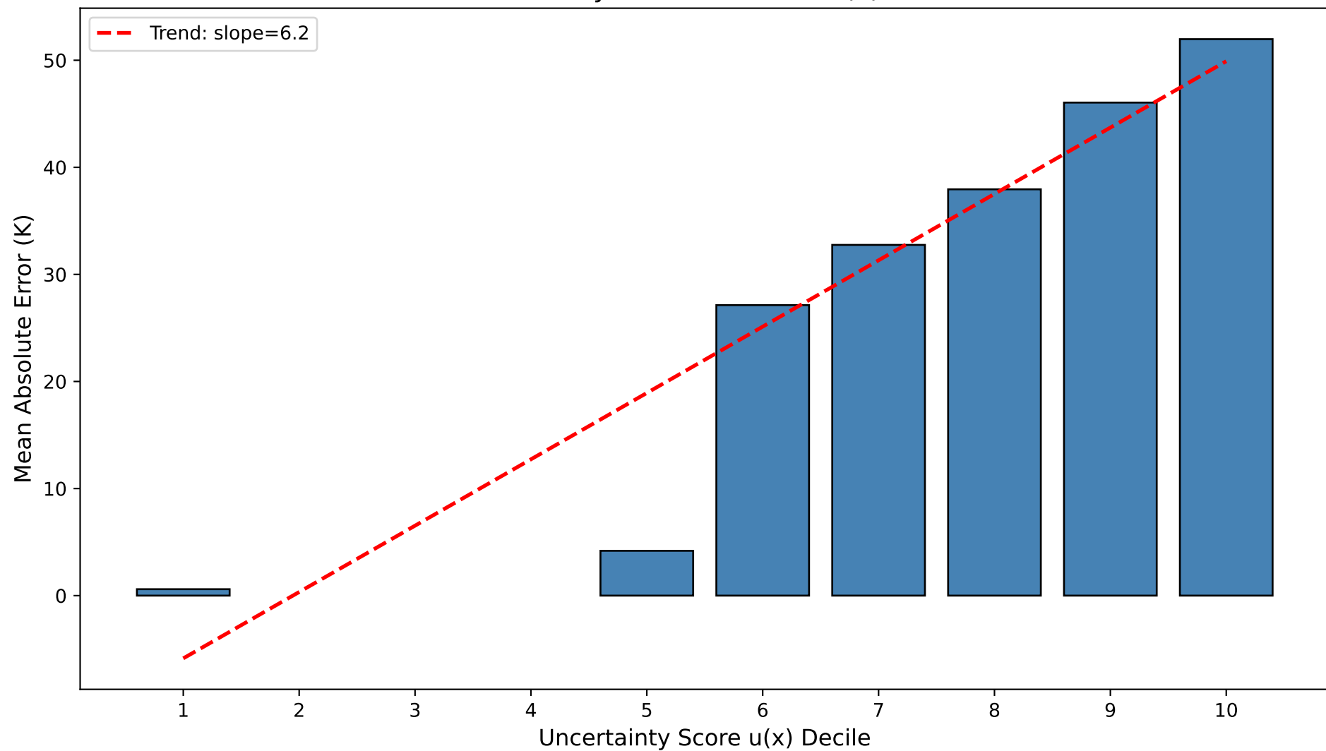
Monotonicity Check: MAE vs. u(x) Decile
