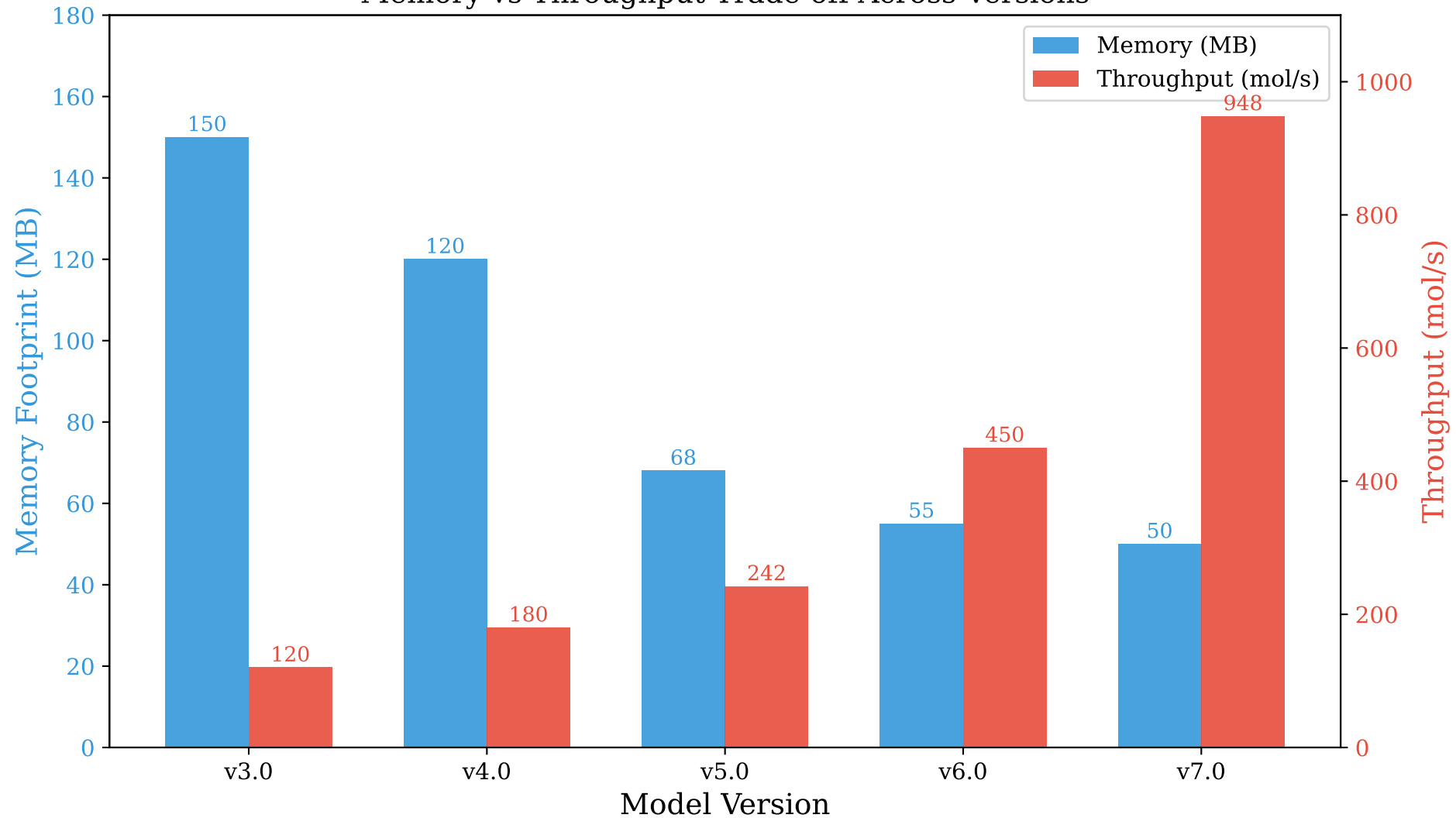
Memory vs Throughput Trade-off Across Versions
