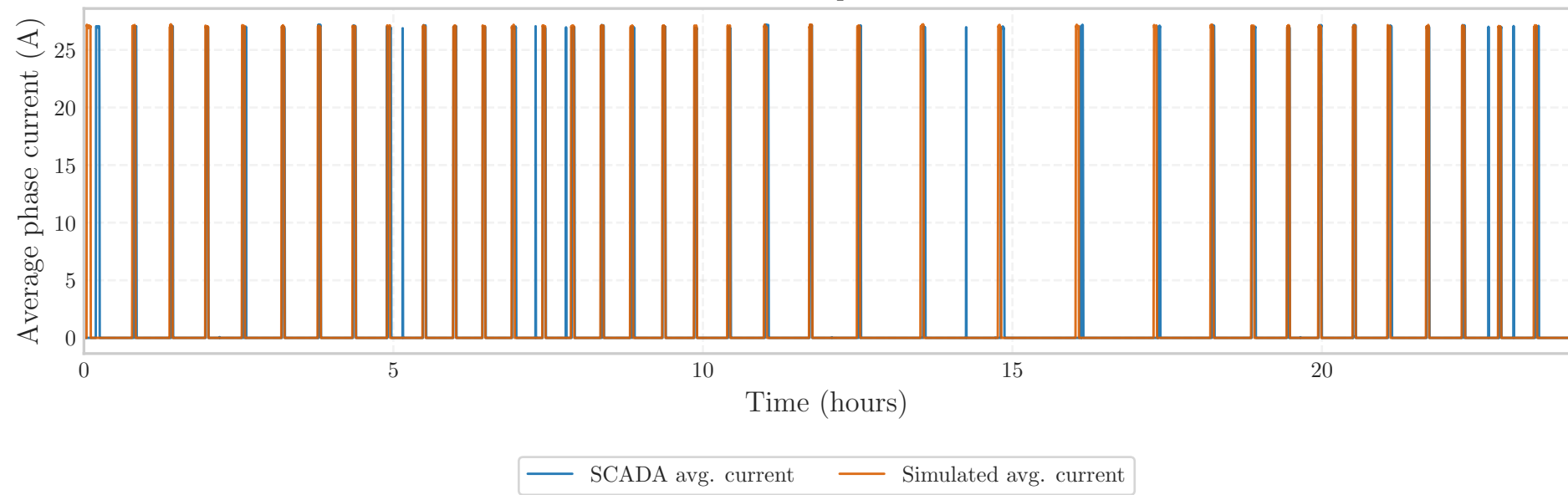
Pump 1
