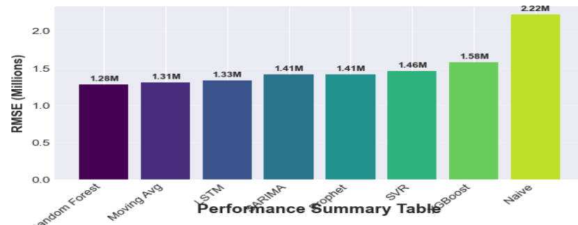
Root Mean Squared Error (Lower is Better)
