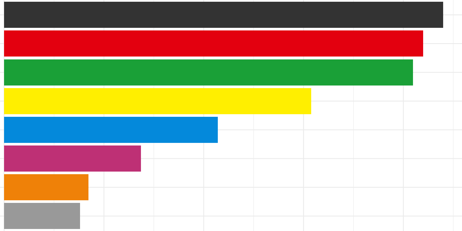
Partei-Scores
