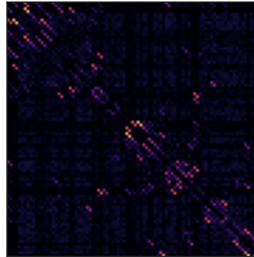
|Empirical - GIN|
