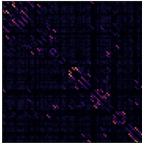
|Empirical - MLP|
