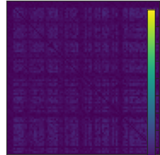
GIN aligned
