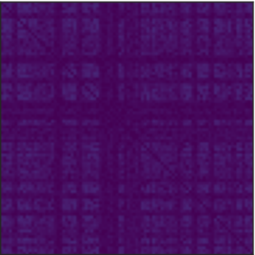
GAT aligned
