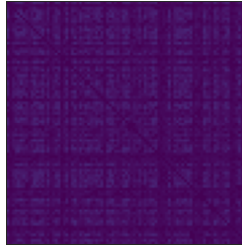
MLP aligned
