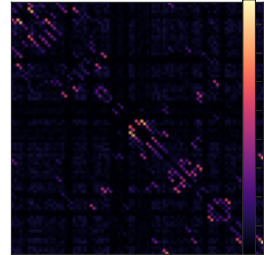
|Empirical - GAT|
