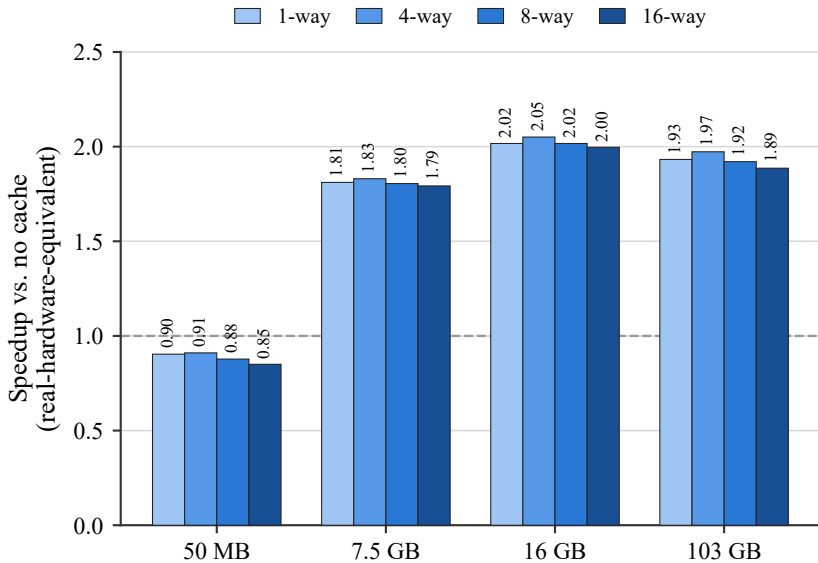
Cache speedup by width and database size
