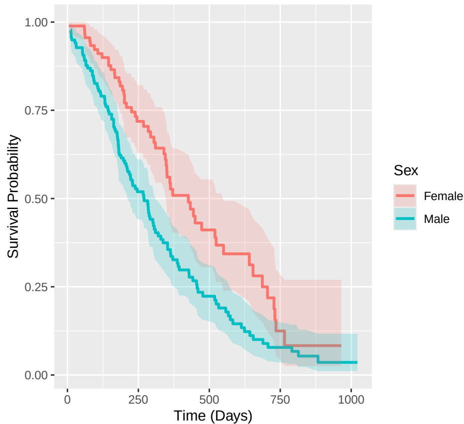
Kaplan–Meier Survival Curves by Sex Lung Cancer Dataset (N=228)
