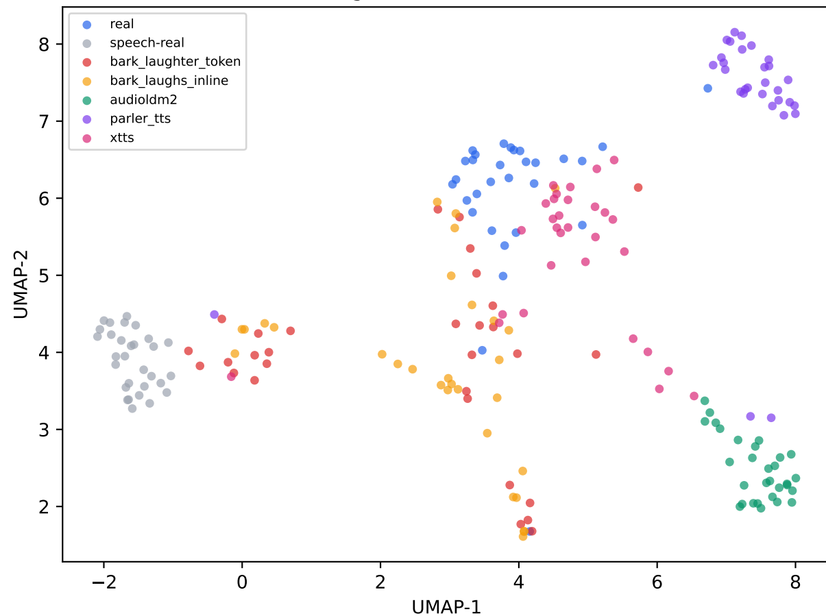
WavLM L9 (length/silence/loudness-controlled)
