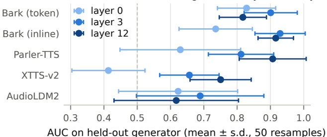
(b) Transfer to a held-out generator, by WavLM layer
