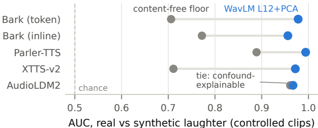
(a) Within-generator probe vs content-free baseline
