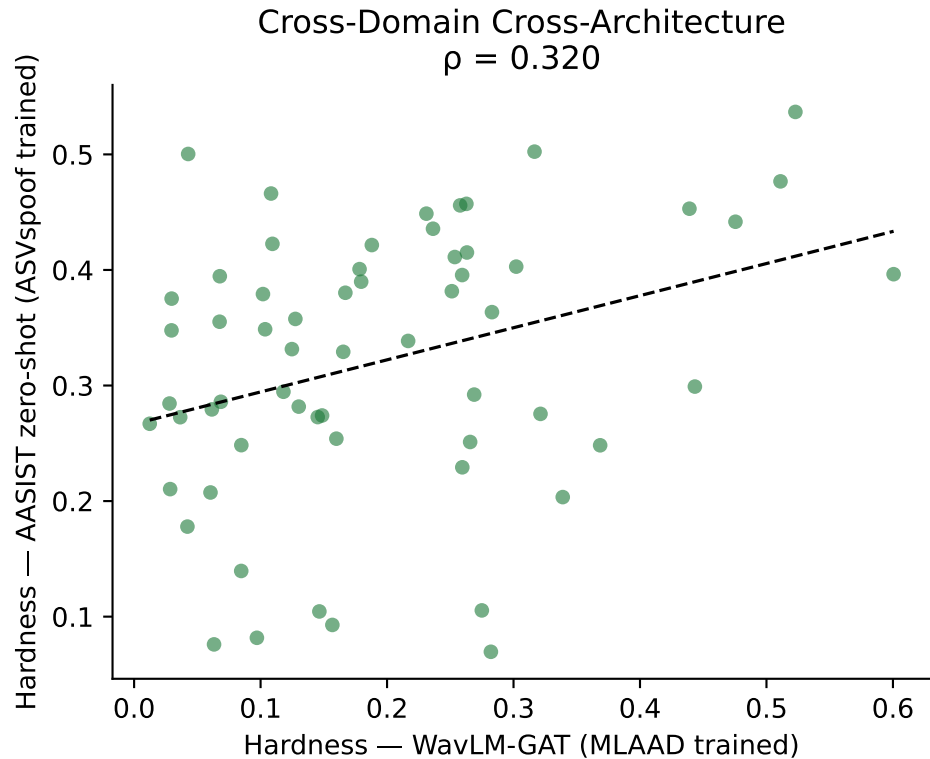
Figure 2: Cross-Detector Hardness Agreement on MLAAD Systems
