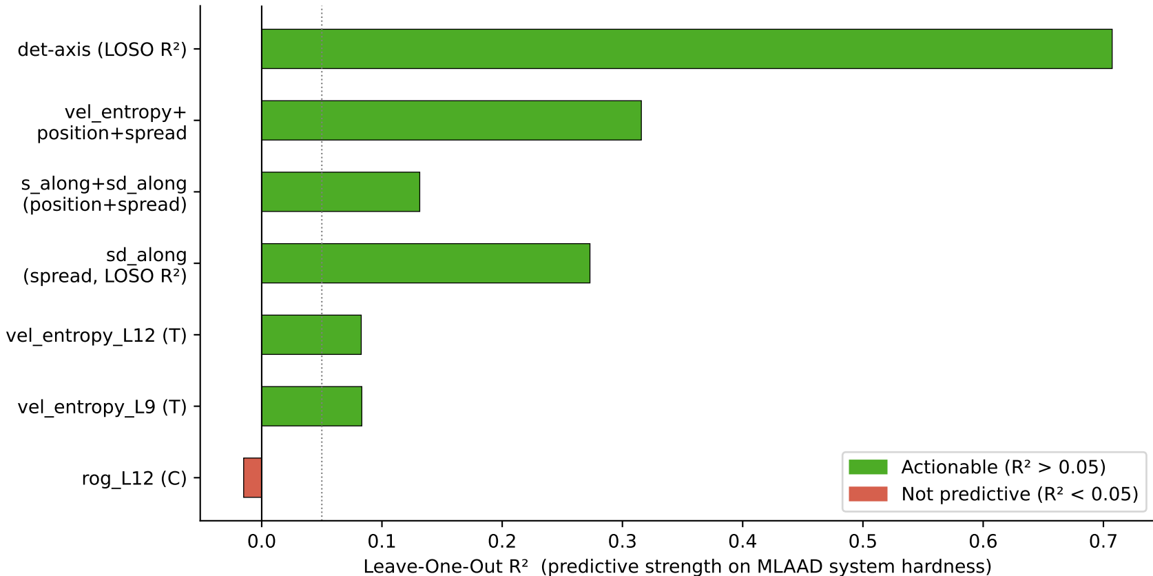
Figure 3: Predictive Strength of Geometry Features (green = actionable, red = noise)
