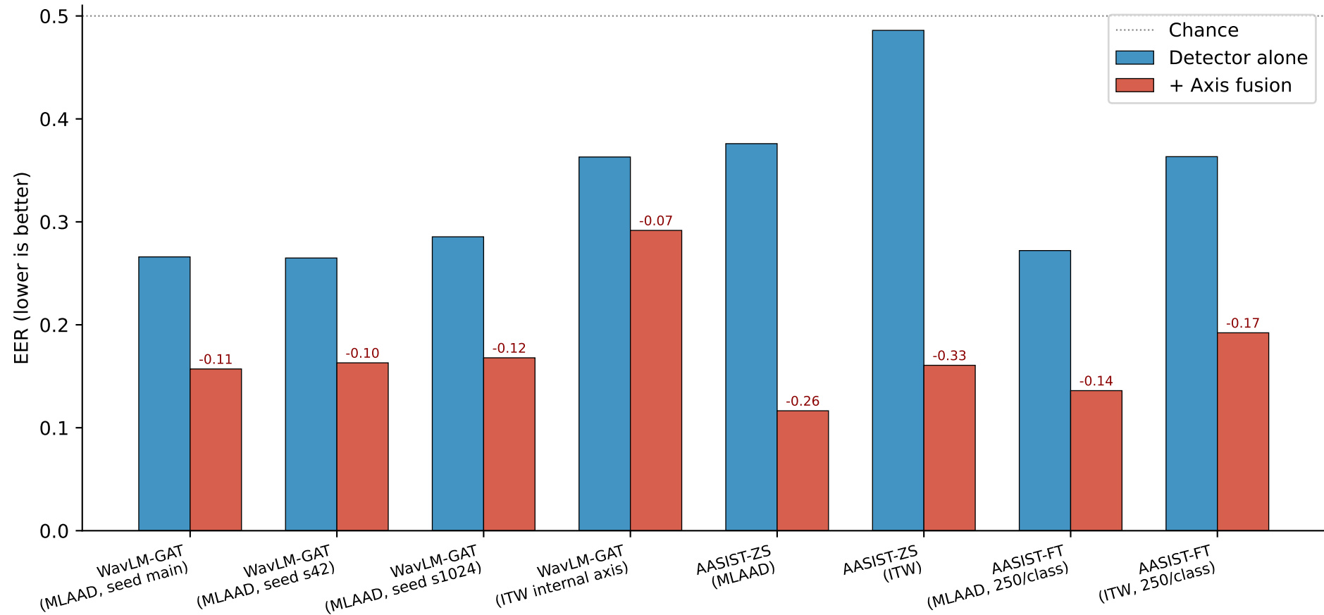
Figure 5: EER Before vs After Axis Fusion Across Detectors and Datasets
