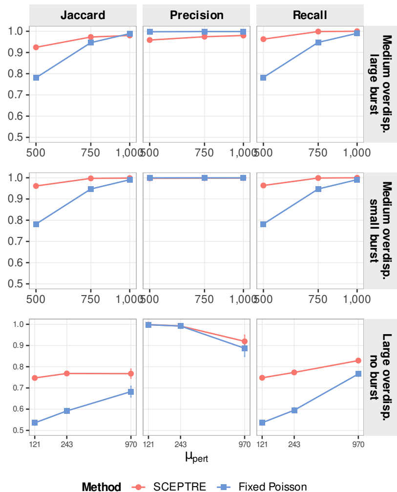
(B) Evaluation of SCEPTRE bug on simulated guides
