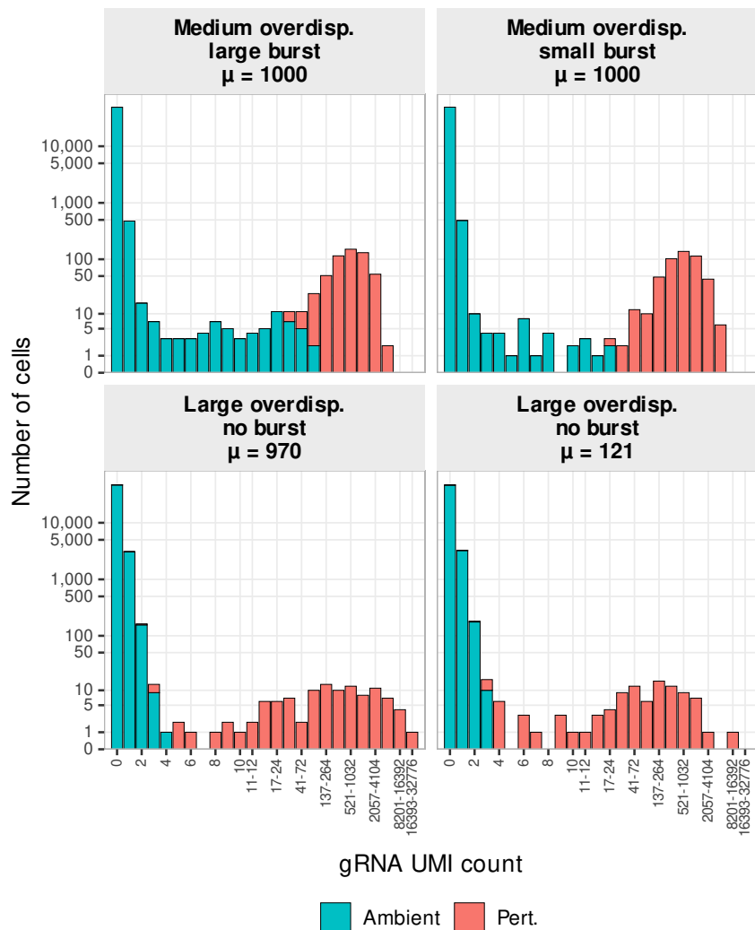
(A) Simulated gRNA counts: ambient vs. perturbed
