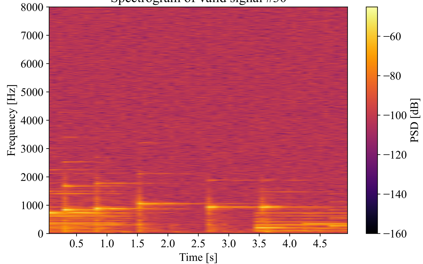
Spectrogram of valid signal #30
