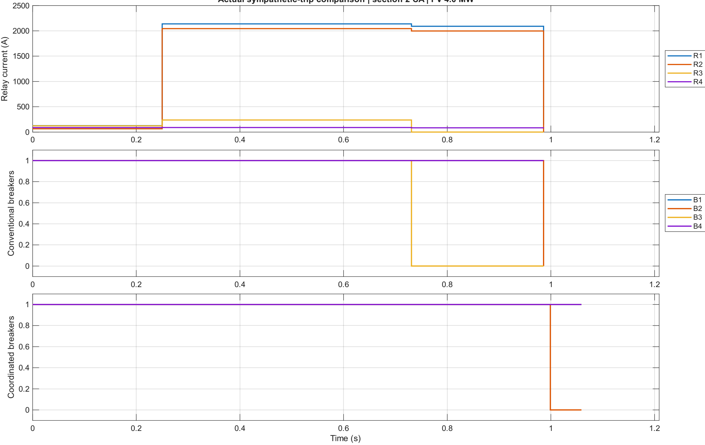
Actual sympathetic-trip comparison | section 2 CA | PV 4.0 MW
