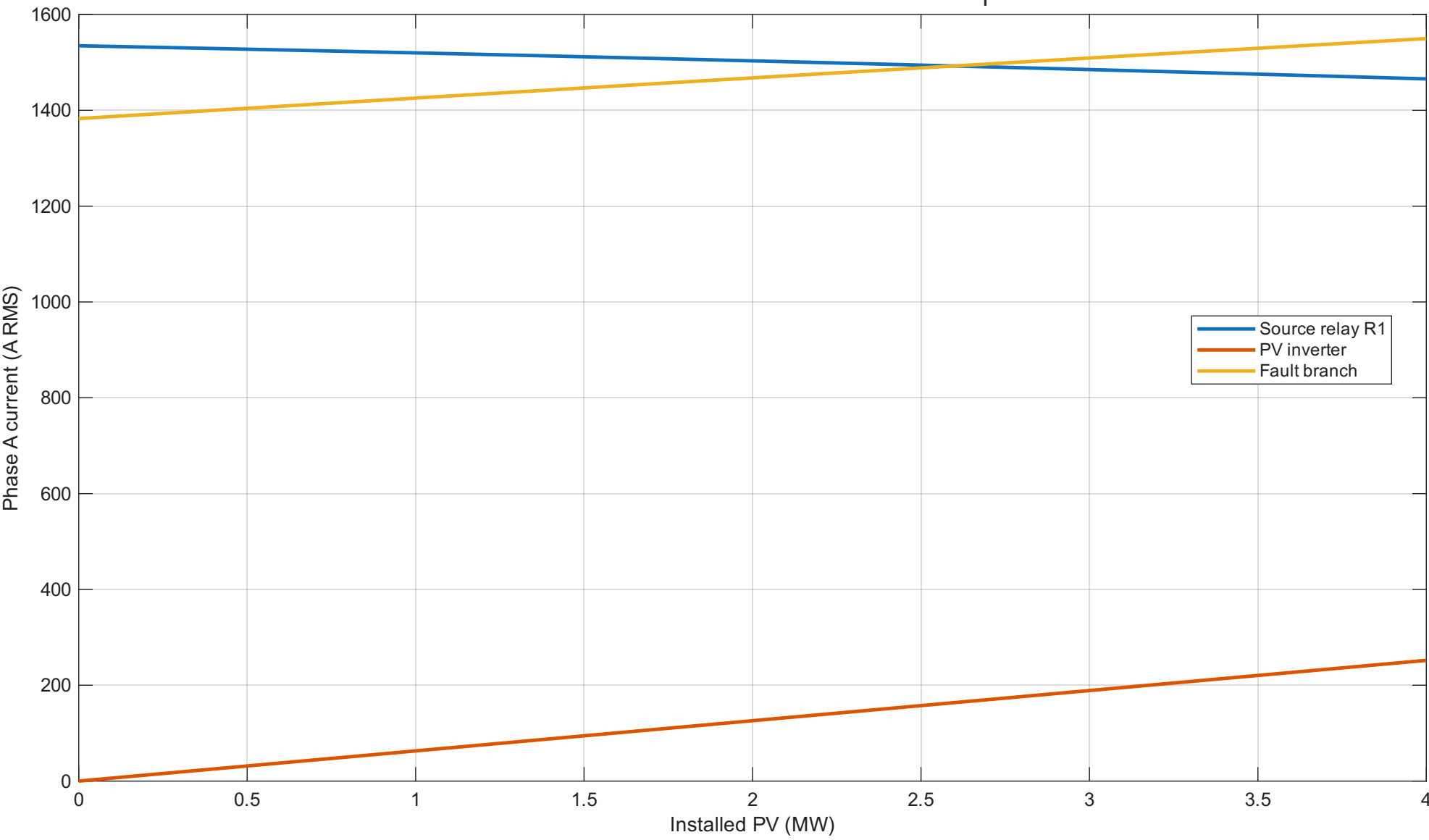
PV fault contribution | section 3, midpoint ABC-G fault, R_f = 2 ohms
