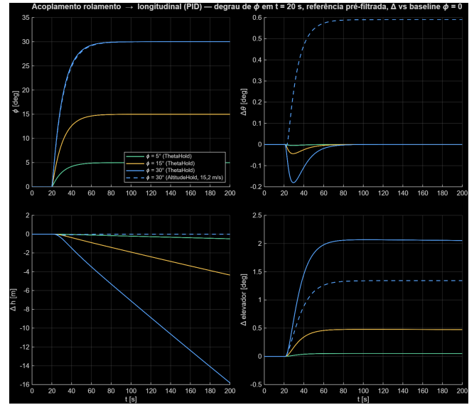
FIGURE 5. Roll-to-longitudinal coupling (PID), amplitude sweep: \phi^{ref} steps of 5/15/30^\circ at t = 20 s, prefiltered reference; \phi , \Delta\theta , \Delta h , and \Delta\text{elevator} relative to the \phi = 0 baseline. Solid: ThetaHold at the 12 m/s trim; dashed: 30^\circ in AltitudeHold at 15.2 m/s. [PENDENTE: re-exportar em fundo branco para a versão final]
