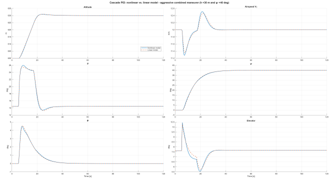
FIGURE 7. PID, aggressive combined maneuver ( h + 30 m and \psi + 40^\circ simultaneous): nonlinear model vs. linear closed loop.
