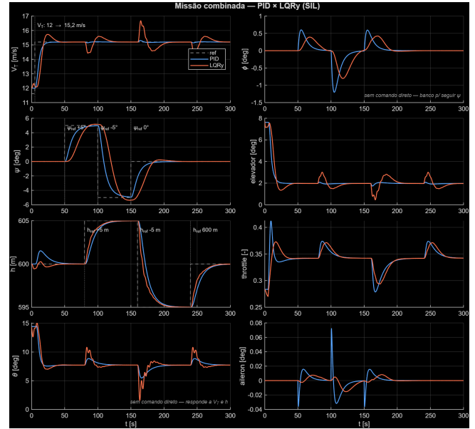
FIGURE 8. Combined mission: PID vs. LQRy on the nonlinear model, identical references — states on the left, actuators on the right. [PENDENTE: re-exportar em fundo branco para a versão final]
