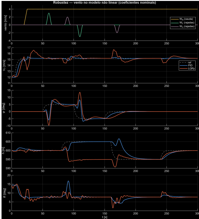
FIGURE 11. Scenario D (wind and gusts): wind profile (NED components) and closed-loop responses. [PENDENTE: re-exportar em fundo branco para a versão final]
