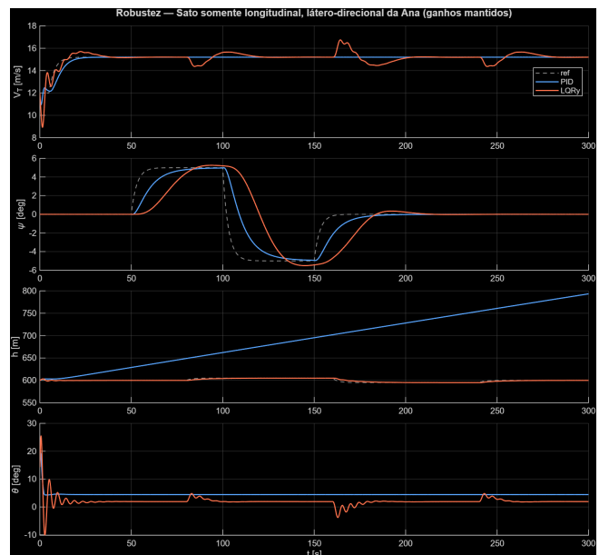
FIGURE 10. Scenario B (longitudinal mismatch only): the PID's altitude hold drifts +193 m while its heading and airspeed stay nominal; the LQRy remains near nominal on every channel. [PENDENTE: re-exportar em fundo branco para a versão final]
