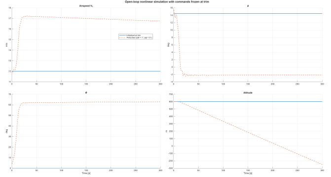
FIGURE 2. Open-loop nonlinear simulation with commands frozen at trim. Solid: initialized exactly at trim (remains at equilibrium). Dashed: small initial perturbation — the unstable spiral mode diverges.
