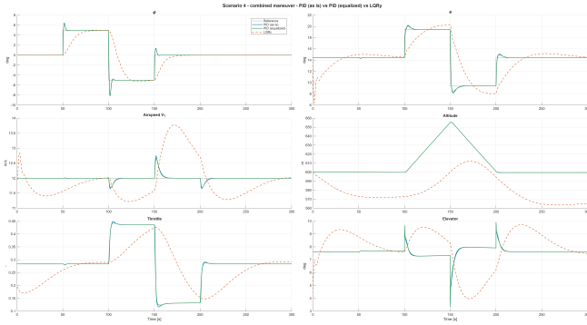
FIGURE 6. Equalization ablation, combined scenario: PID as delivered vs. PID with the harness equalized to the LQRy rig (24 rad/s actuators, no rate limits, no clamp, no prefilter), with the LQRy response for context.
