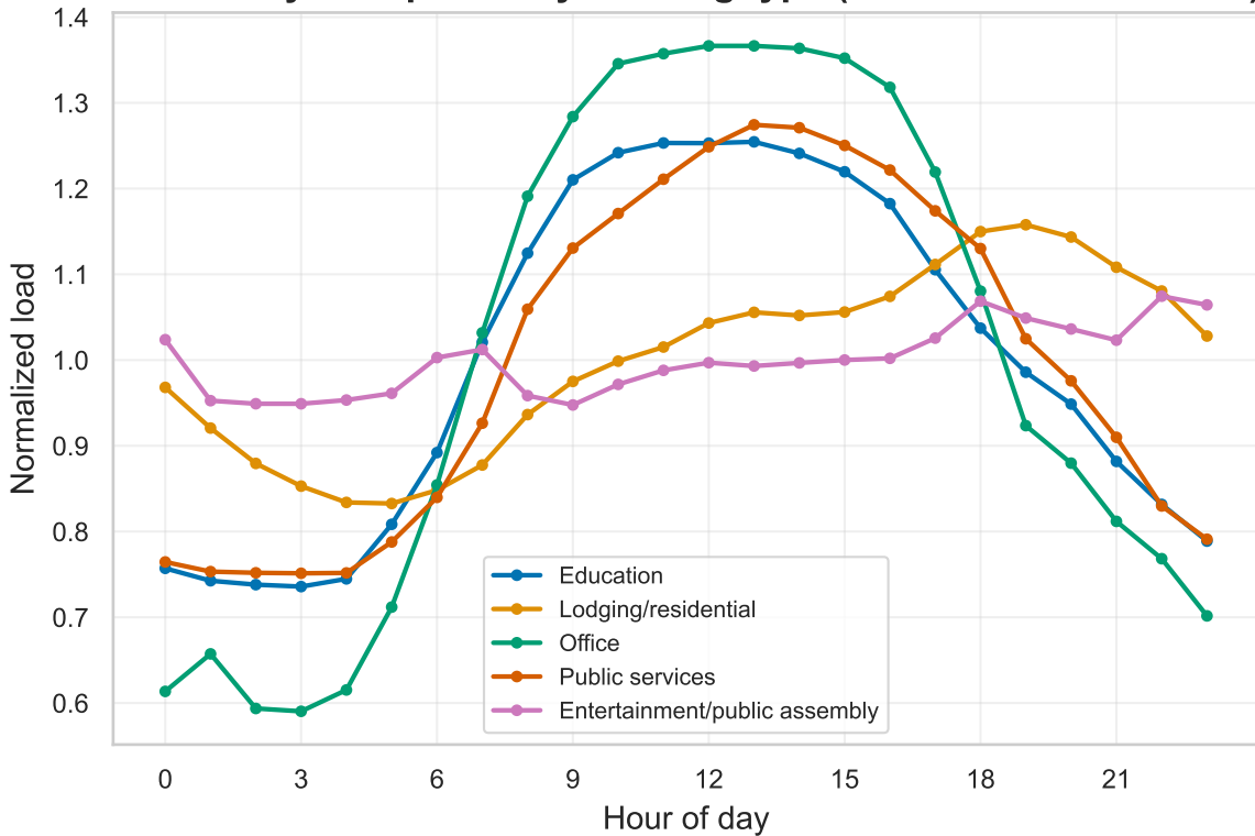
Mean daily load profile by building type (own-mean normalized)
