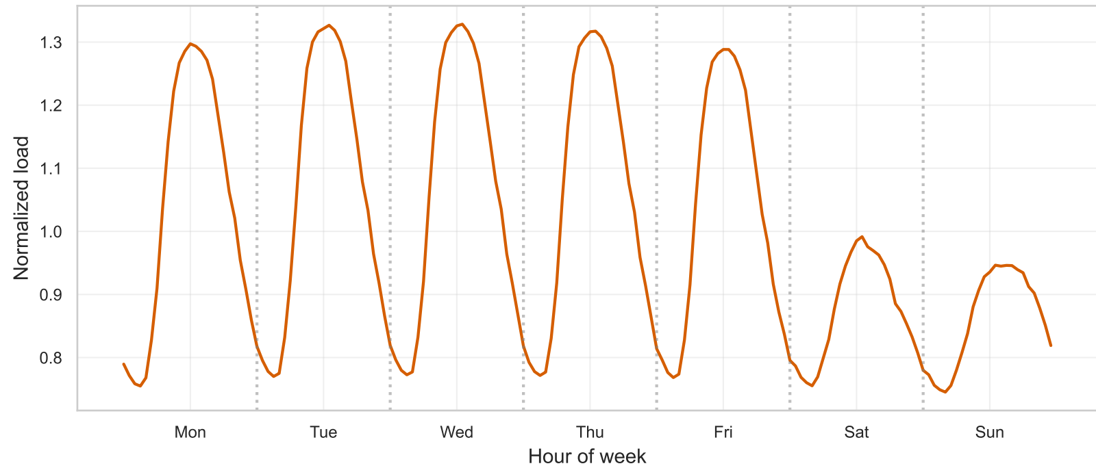
Mean weekly load profile (Mon-Sun)
