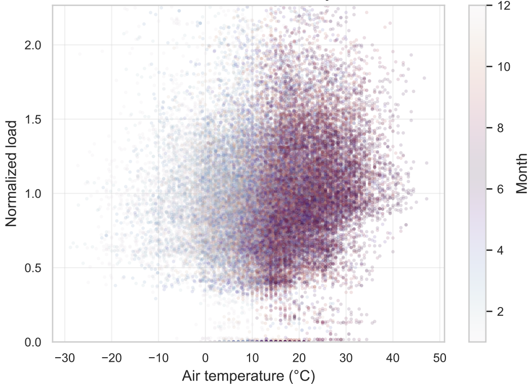
Normalized load vs air temperature
