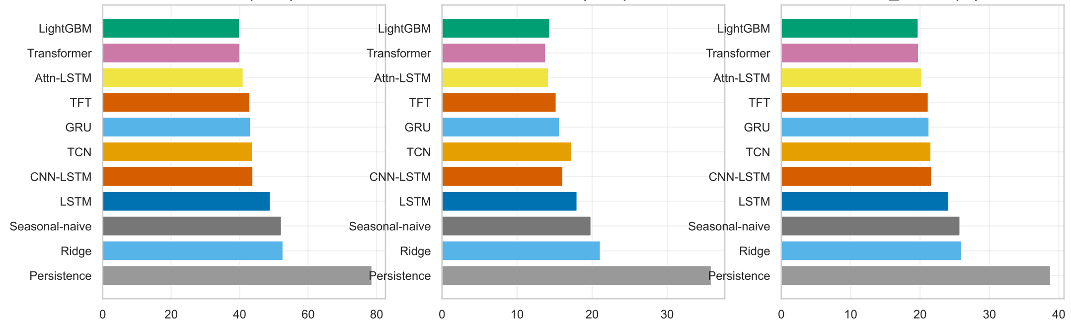
Model comparison on BDG2 test set (24 h horizon) MAE (kWh)
