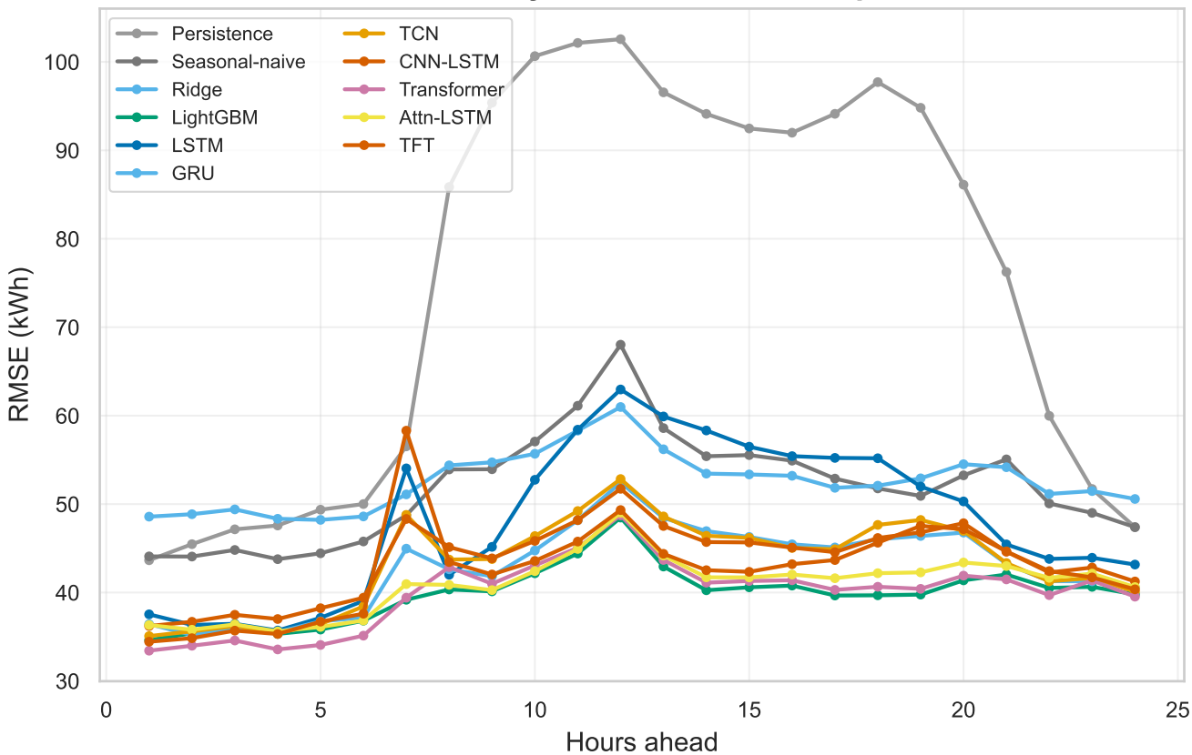
RMSE by forecast horizon step
