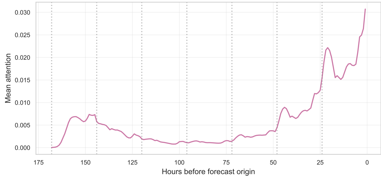
attn_lstm attention vs lag (test set)
